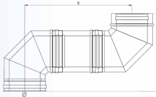
ELBOW 90° WITH PIECE 0.25m
