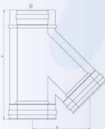
TEE 135°
