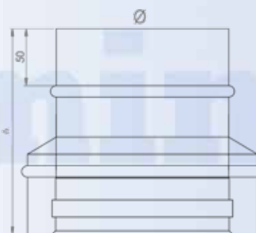
ADAPTOR SW TO DW
