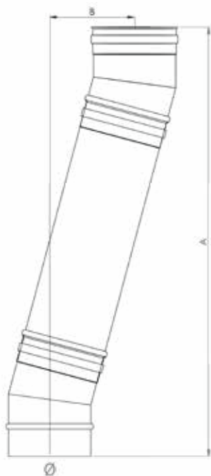
ELBOW 15° WITH PIECE 0.50m
