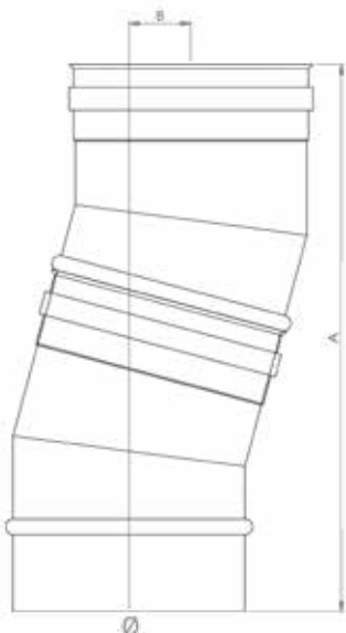
ELBOW 15°
