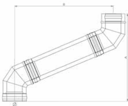
ELBOW 67° WITH PIECE 0.50m
