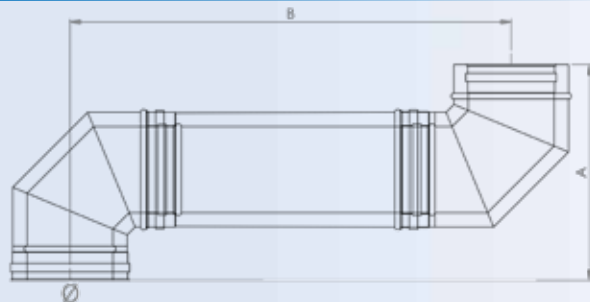
ELBOW 90° WITH PIECE 0.50m
