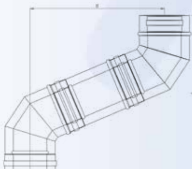
ELBOW 67° WITH PIECE 0.25m
