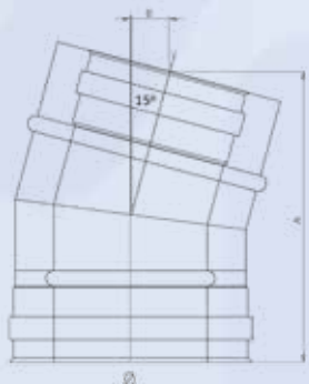
ELBOW 15°
