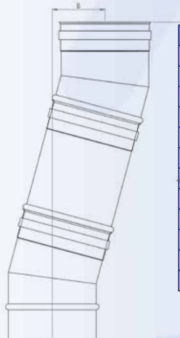
ELBOW 15° WITH PIECE 0.25m
